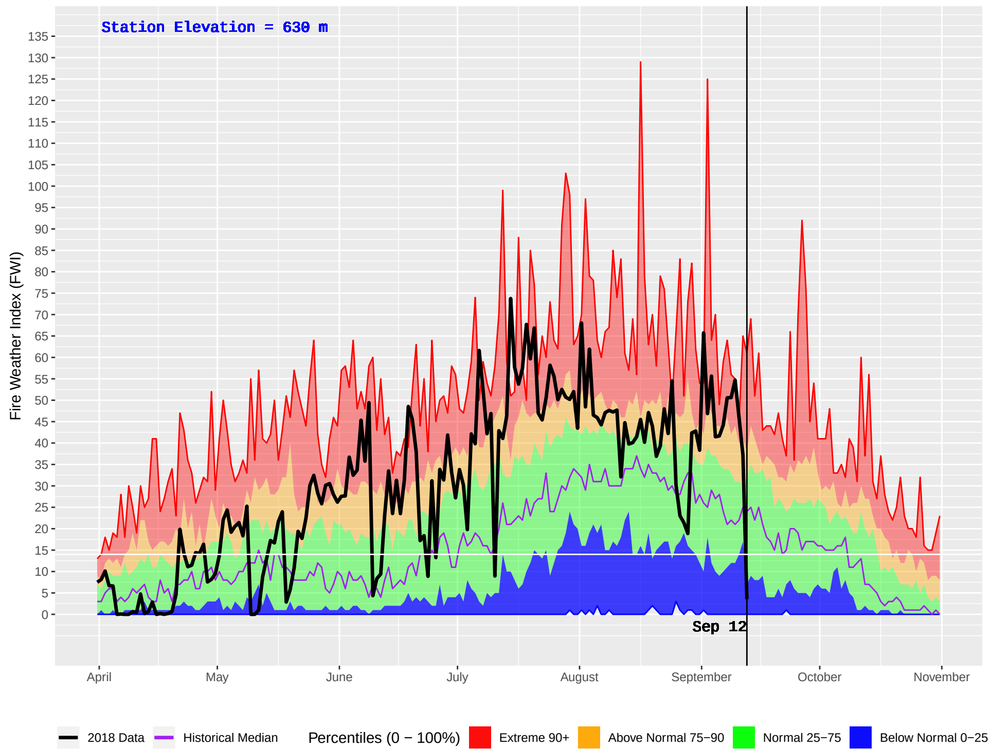
GRAND FORKS (392) : Historical (1981–2016) and Current (2018) Daily Fire Weather Index (FWI)
